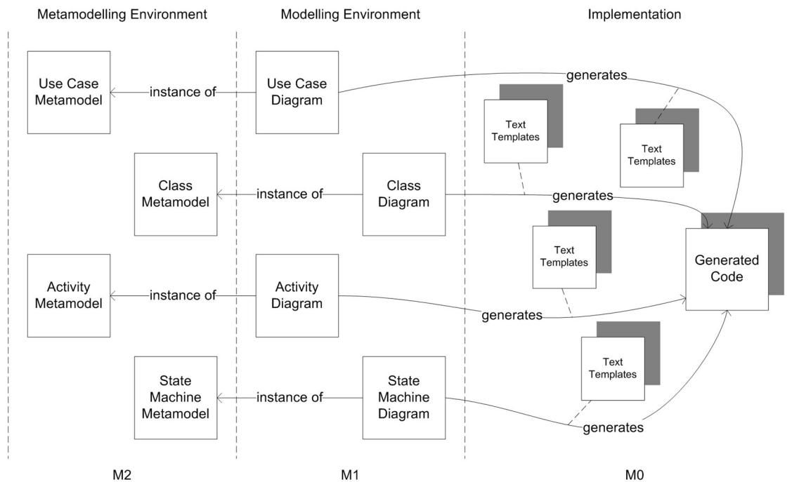
Figure 22 – Layered modelling architecture of Microsoft DSL Tools
