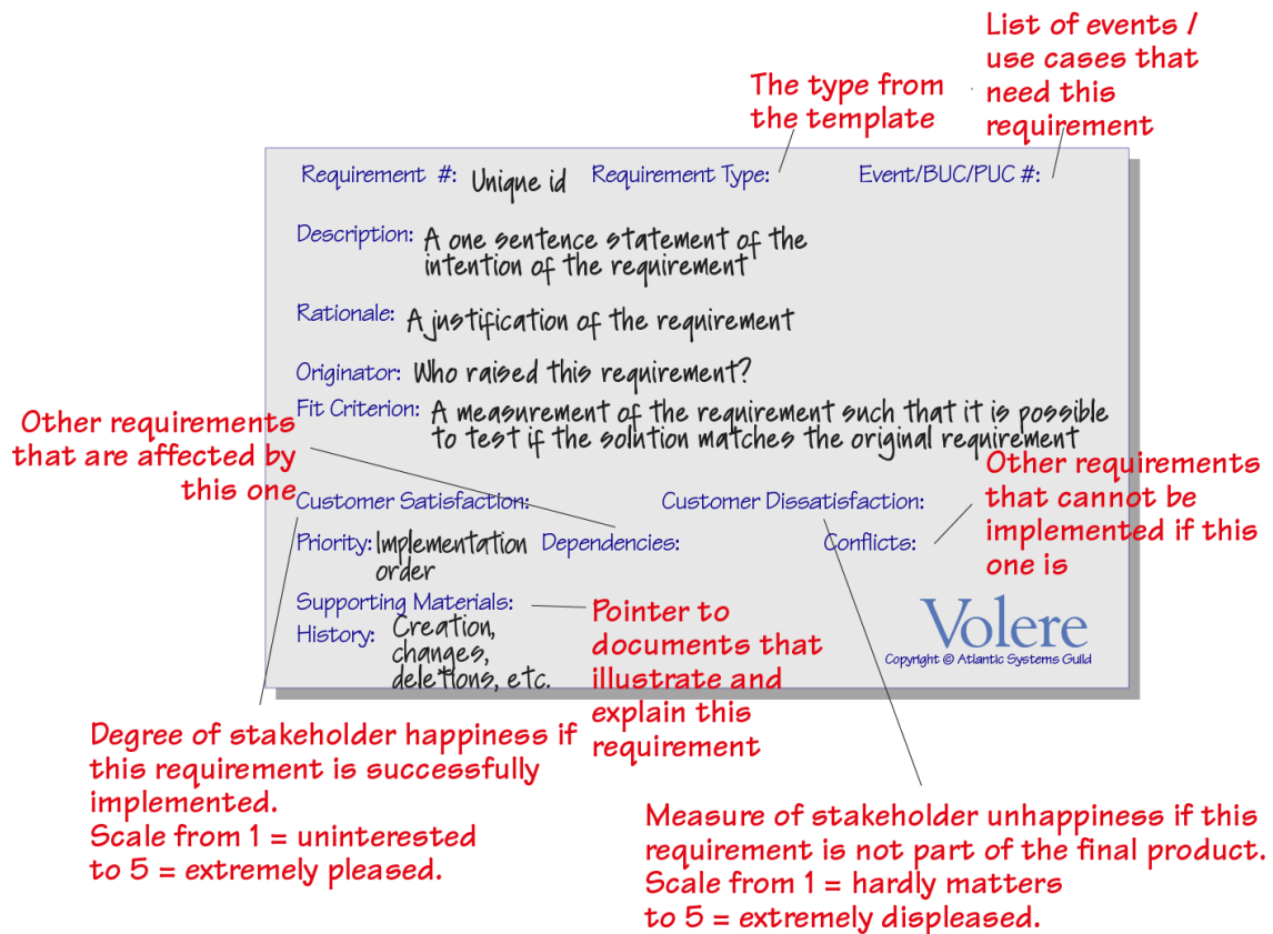
Figura 3.5 - Requirements Shell [62]
